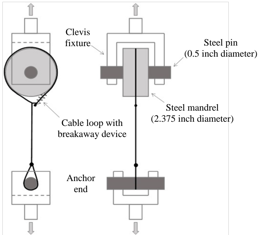
Figure 1: Test fixture, side and front views.
